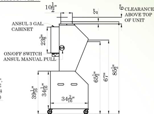
LEFT SIDE ELEVATION VIEW
