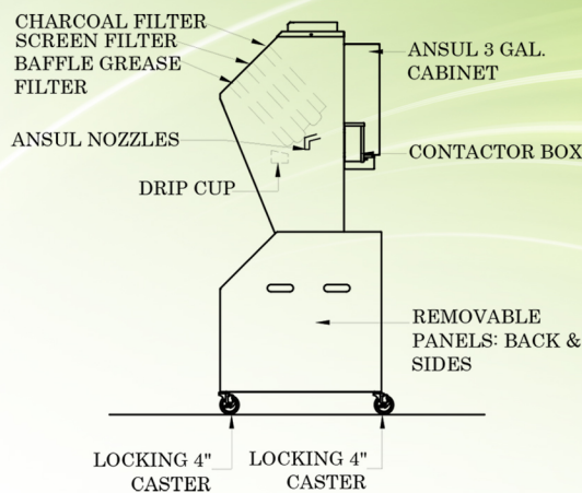
RIGHT SIDE ELEVATION VIEW
