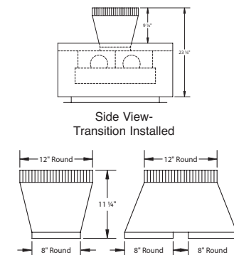
VP564 Standard Transition (Included)
