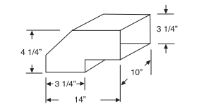
Optional VP559 back vent elbow is available for back vent applications
