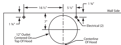
Top View- Two B200 Dual Blowers 1200 CFM
