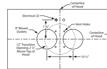
Top View- T400 Cluster Blower 1100 CFM
