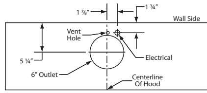
Top View- B100 Single Blower 300 CFM
