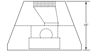
Side View- Transition Installed
