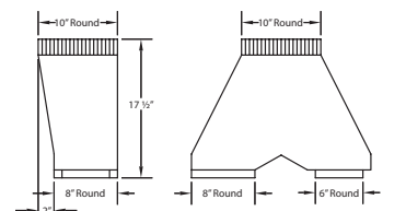
VP562 Transition (Optional) for B200 Dual & B100 Single Blower
