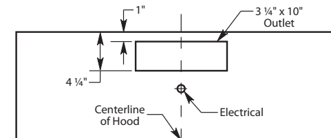
K250 Ceiling Cutout For Vertical Ducting Viewed From Above
