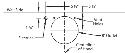
Top View- B200 Dual Blower 600 CFM
