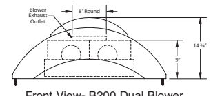
Front View- B200 Dual Blower
