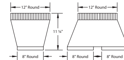
VP564 Standard Transition (Included)
