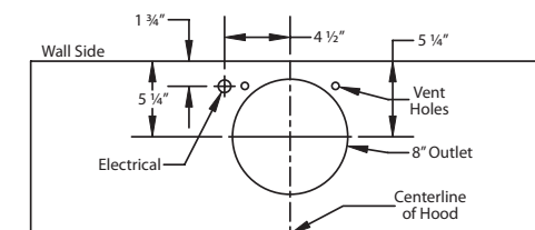
Top View- B200 Dual Blower 600 CFM
