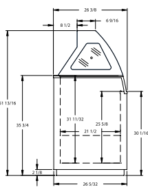
CURVED GLASS SIDE VIEW
