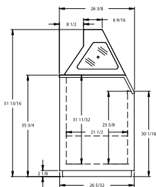
STRAIGHT GLASS SIDE VIEW
